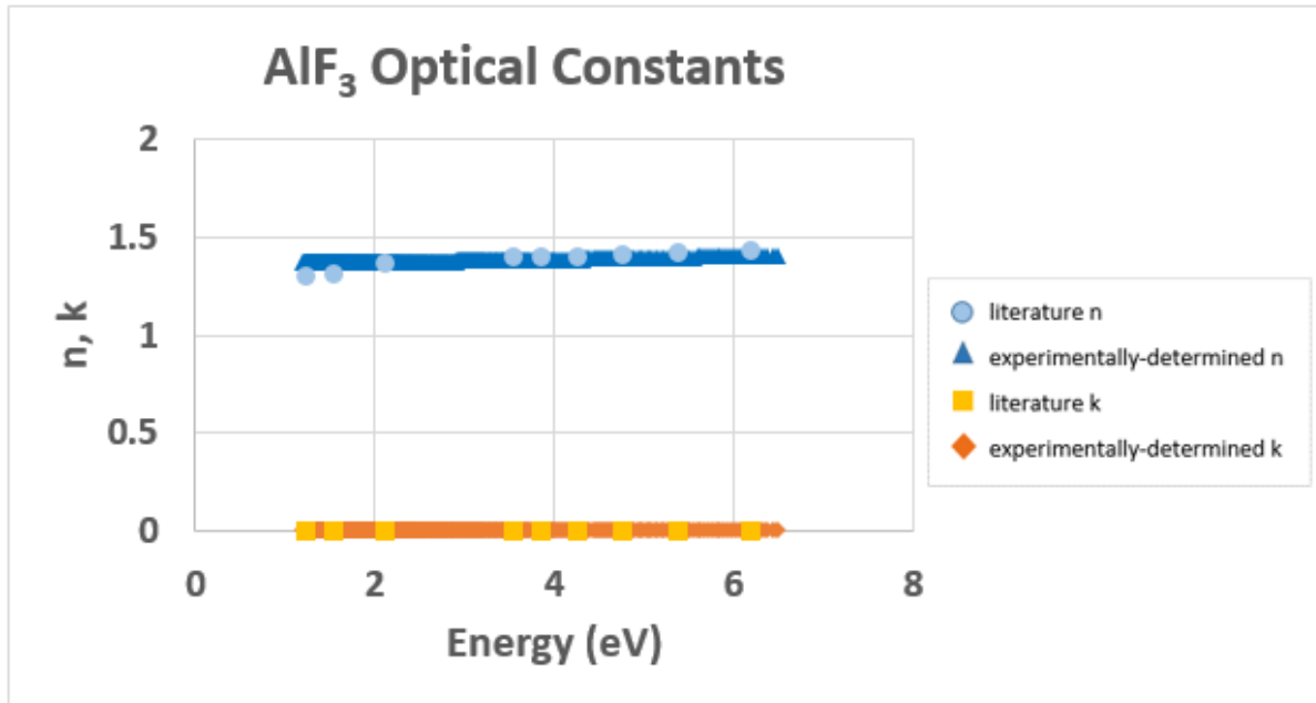
Figure 21: Optical constants for AlF 3 as determined by ellipsometric fitting as compared to optical constants from literature 12 . n and k are the components of the complex index of refraction where index = n + i k.
